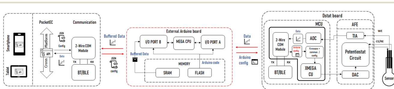
Fig. 6 Block diagram for DStat measurements setup. The red areas indicate the additions made to the previous architecture.
